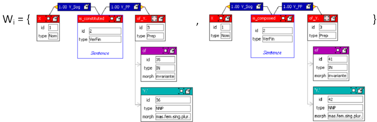
Figure 4: Example of an equivalence class
