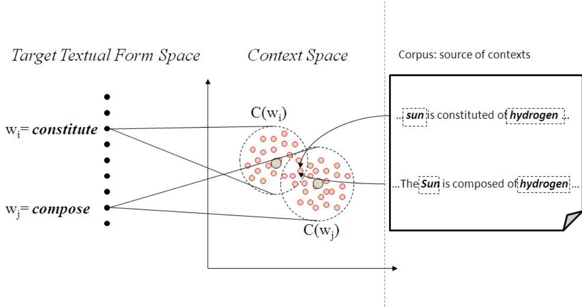
Figure 1: Two spaces for the three hypotheses
