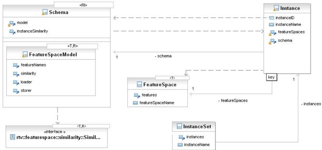
Figure 2: Partial classes diagram of the feature space objects.
